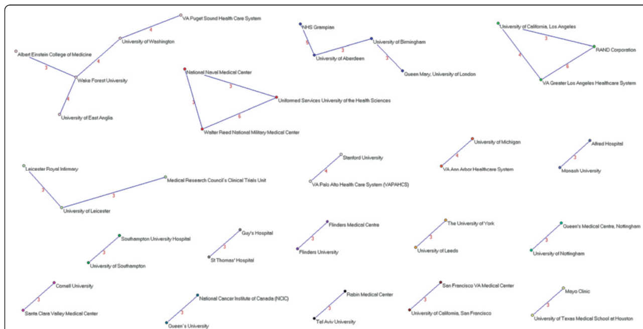
Figure 9 Institutional networks. Other relevant clusters of institutions applying a threshold of three or more papers signed in co-authorship.
