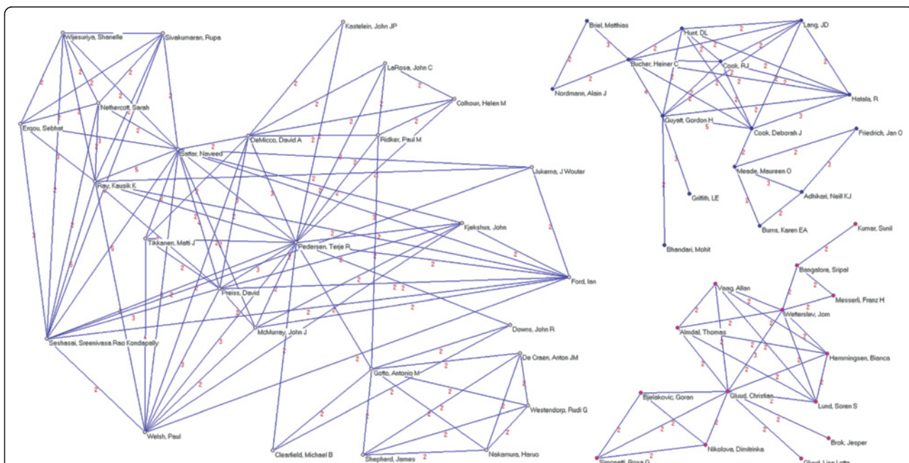
Figure 4 Co-authorship networks. Main clusters of authors ( \geq 15 members), applying a threshold of two or more papers signed in co-authorship.
